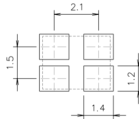
Reference Footpoint
